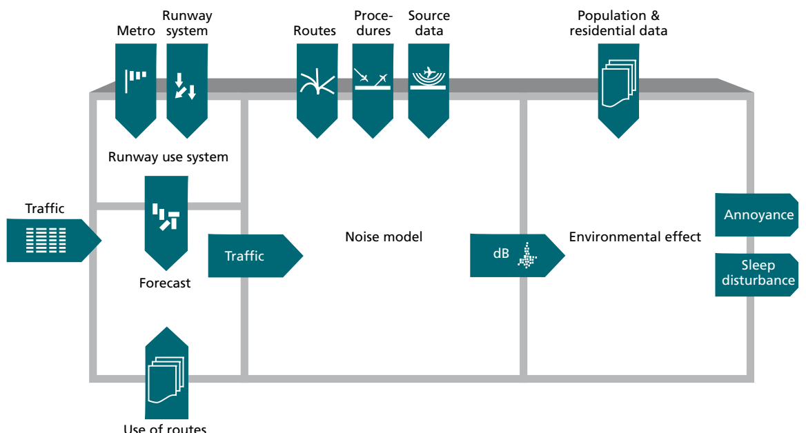
Figure 3. Aircraft noise model (Source To70)
